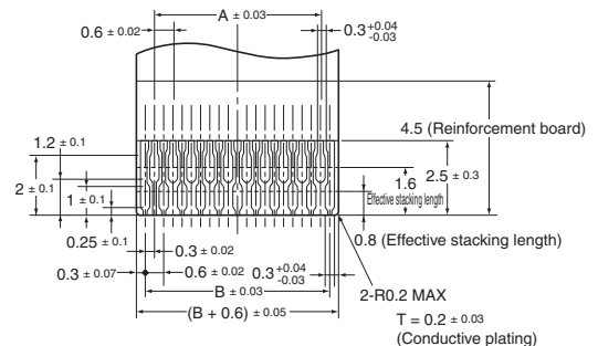
Recommended FPC Dimensions
