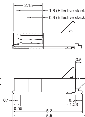
Cross-section diagram: X-X
